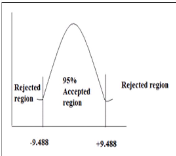
Fig 4: ANOVA: F-Distribution
