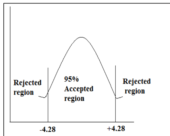
Fig 3: F- Distribution for 100ppm and 50ppm Samples
