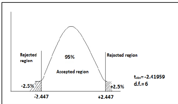
Fig 1: t-Distribution for Two-Tailed Test
